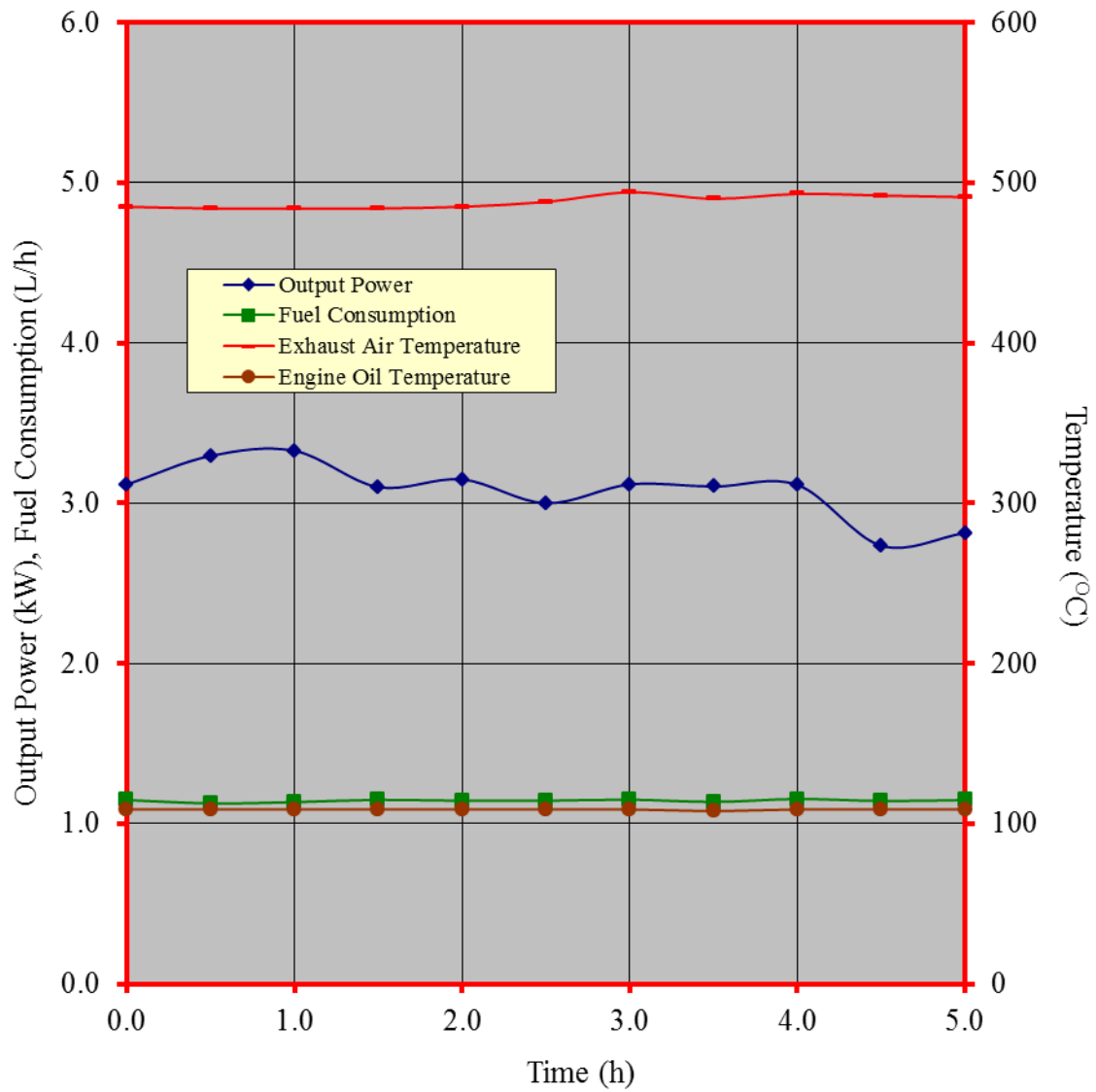
Figure 4. Performance characteristic curves during the continuous running test of the BRIGGS & STRATTON, VANGUARD 13H332 gasoline engine
