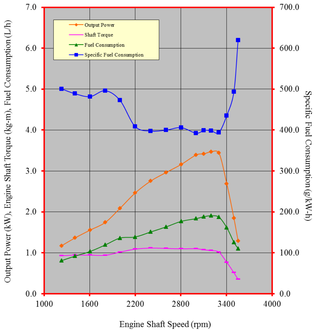
Figure 3. Performance characteristic curves of the BRIGGS & STRATTON, VANGUARD 13H332 gasoline engine
